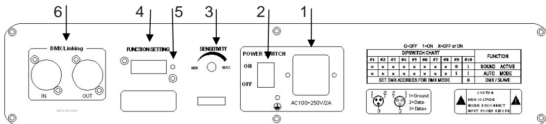
Painel Traseiro
